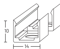
Flexible Aluminium Profile
