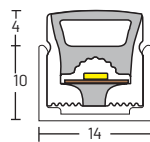
Aluminium Profile
