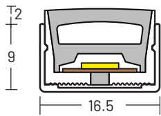
Aluminium Profile (Extrusion: AE1710)
