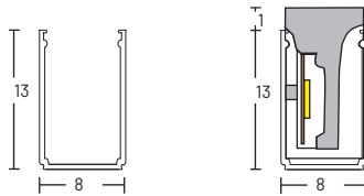
Aluminium Profile
