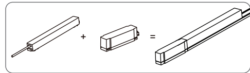
Built-in Driver + Cable Storage MT-SUT23-100W/200W + MT-SUT23-LB
